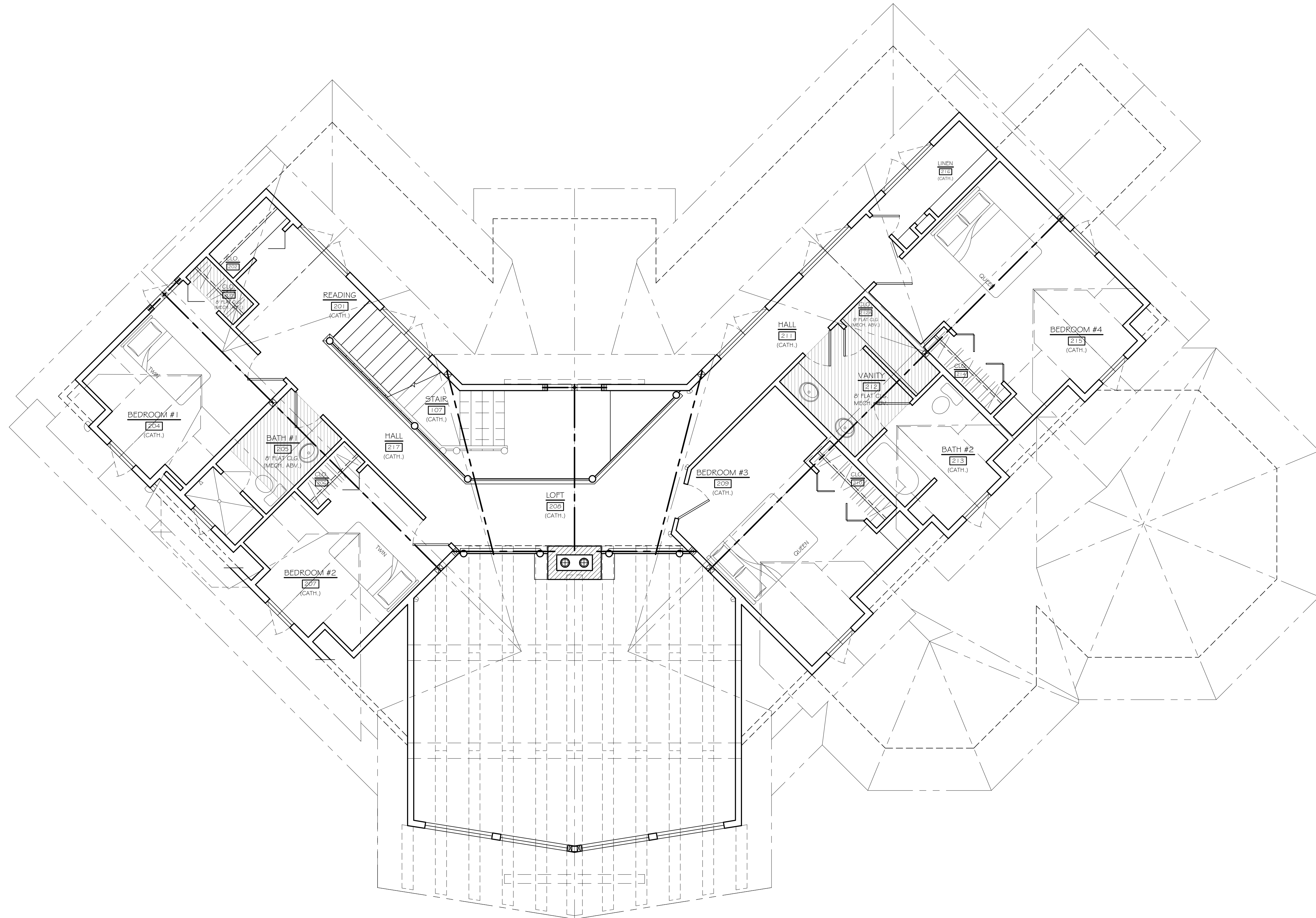
SECOND FLOOR REFERENCE PLAN SCALE: 1/4" = 1'-0"
