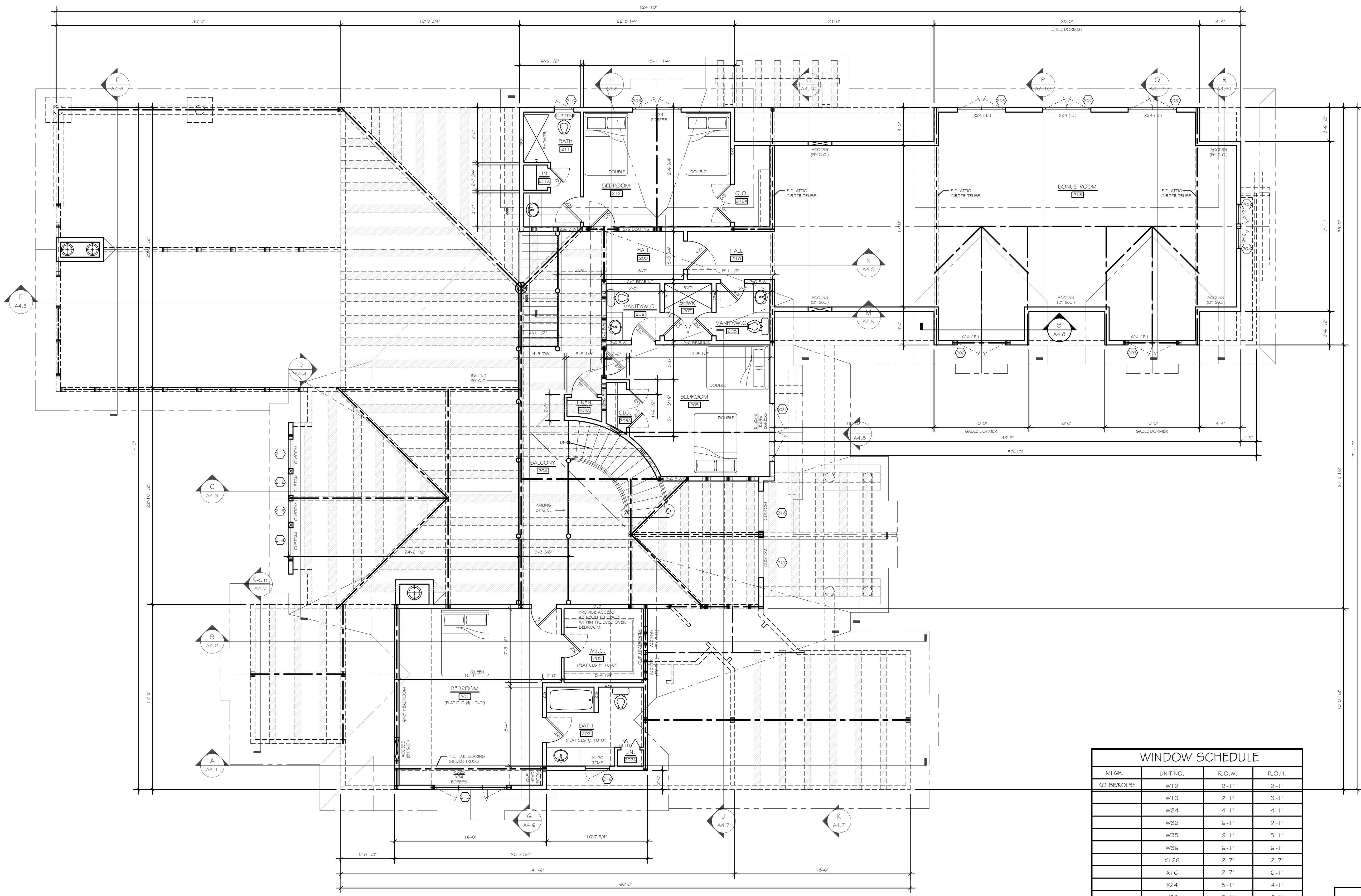
SECOND FLOOR PLAN SCALE: 3/16" = 1' - 0" 1,515 SQ. FT. (LIVING AREA) 1,053 SQ. FT. (BONUS ROOM)
